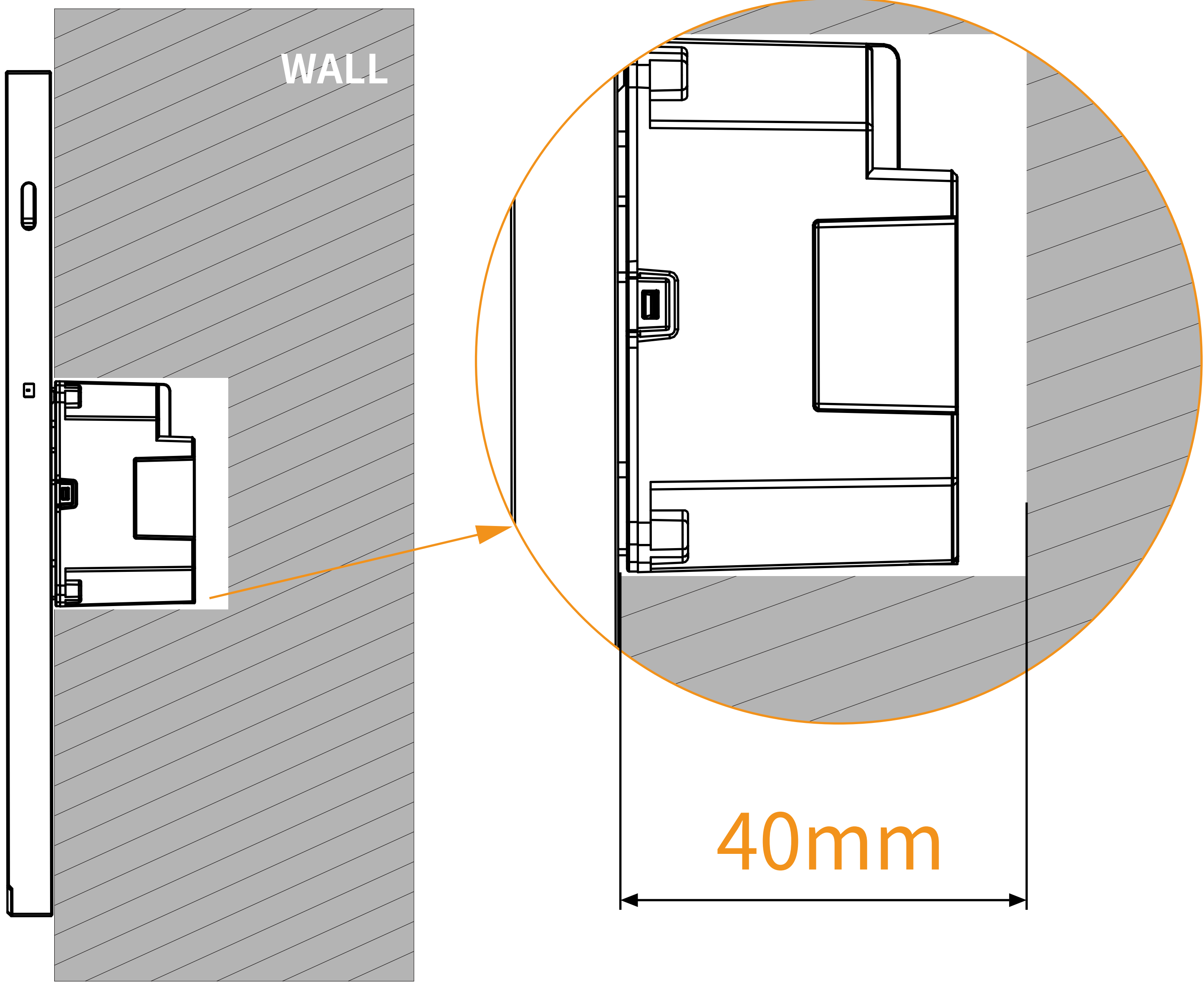
2 SIDE VIEW: HYPANEL SUPREME IN WALL
